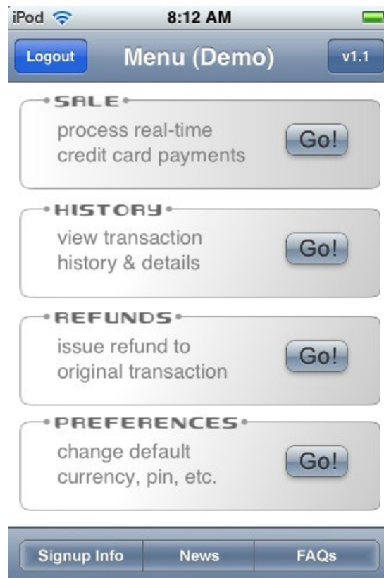
Figure 2. Menu
