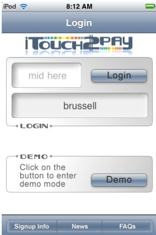
Figure 1. Login screen
